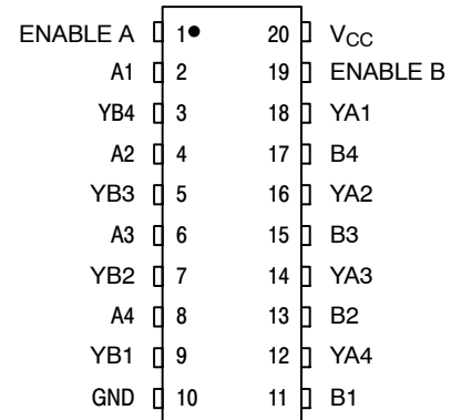
SOIC-20 DW SUFFIX CASE 751D
