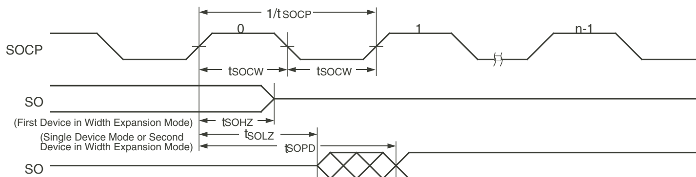
Figure 3. Read Operation
