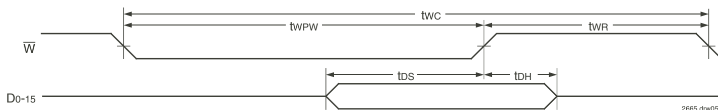
Figure 2. Write Operation
