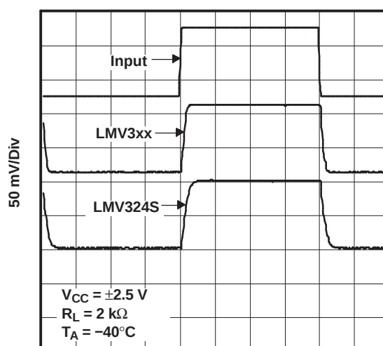
1 \mu\text{s}/\text{Div} Figure 32.
