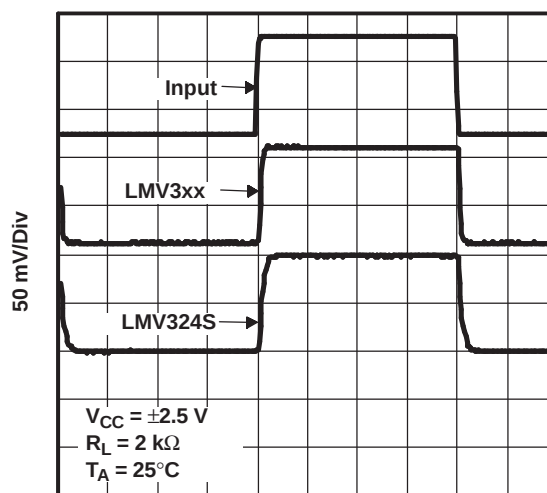
1 \mu\text{s}/\text{Div} Figure 30.
