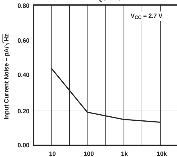
INPUT CURRENT NOISE vs FREQUENCY
