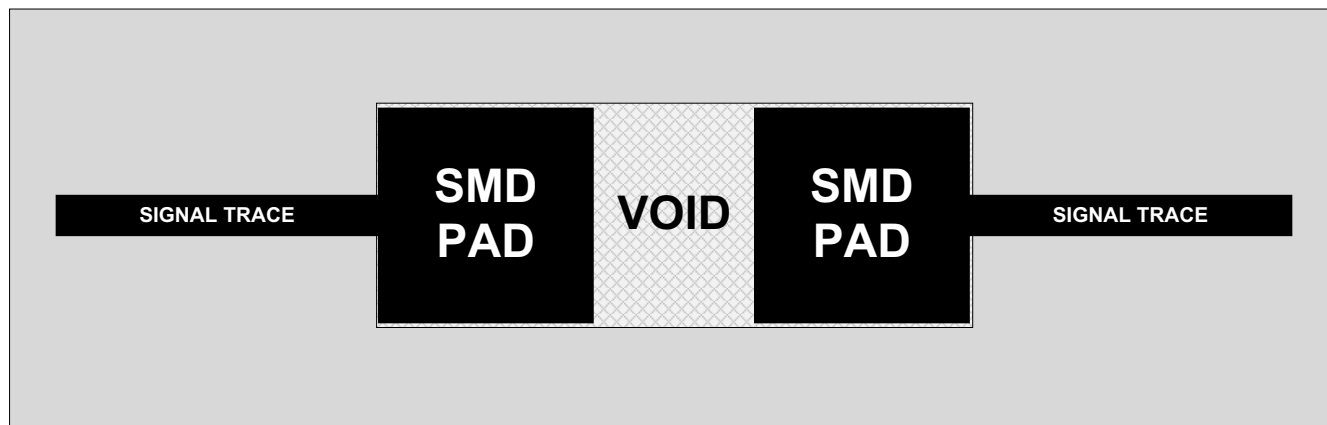
Figure 9-8. Reference Plane Voiding of Surface-Mount Devices
