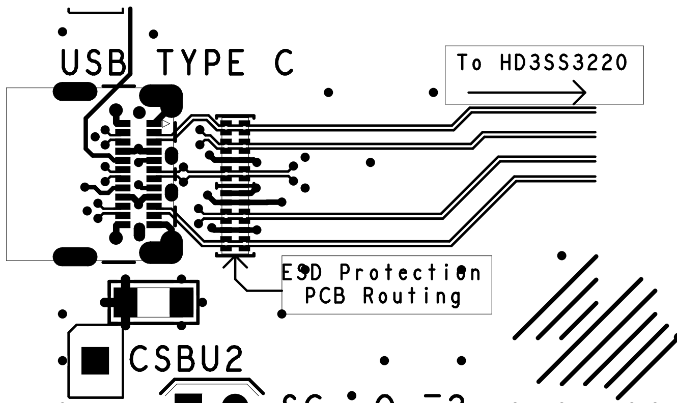
Figure 9-11. Layout Example 2
