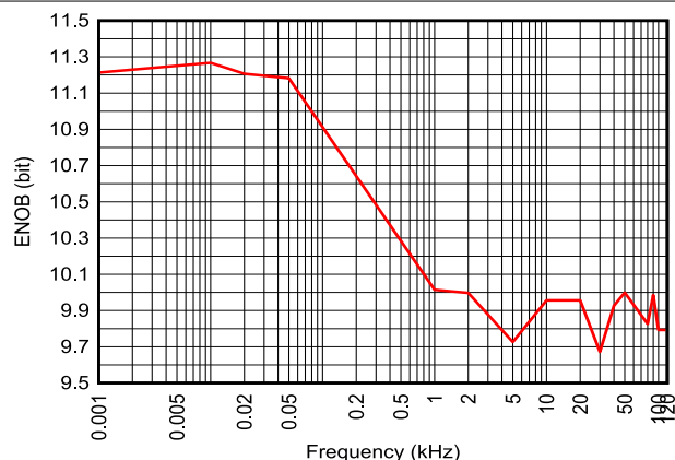
Figure 7-29. ENOB vs. Input Frequency (External Reference = 3.0V)
