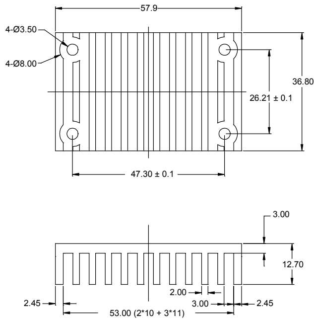
Figure 17 Heatsink
