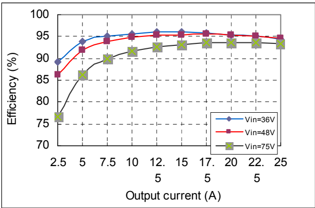
Figure 1 Efficiency vs. output current, T a =25°C, V o =12V
