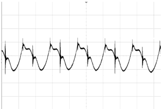
Figure 2 Output ripple & noise (2μs/div, 20mV/div), see Figure 14 for test configuration
