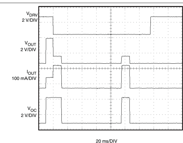
Figure 21. t_{RESTART} Response
