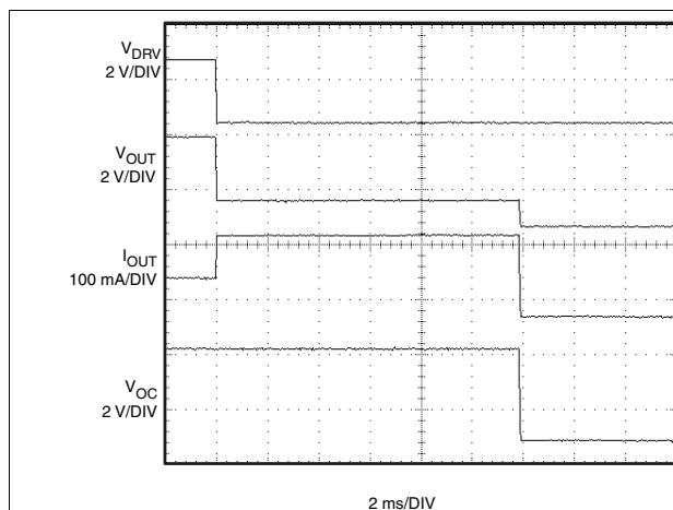
Figure 20. t_{BLANK} Response
