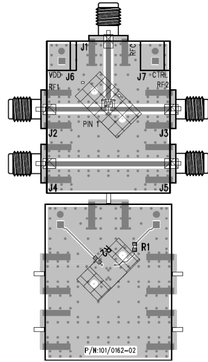
Figure 11. Evaluation board layout
