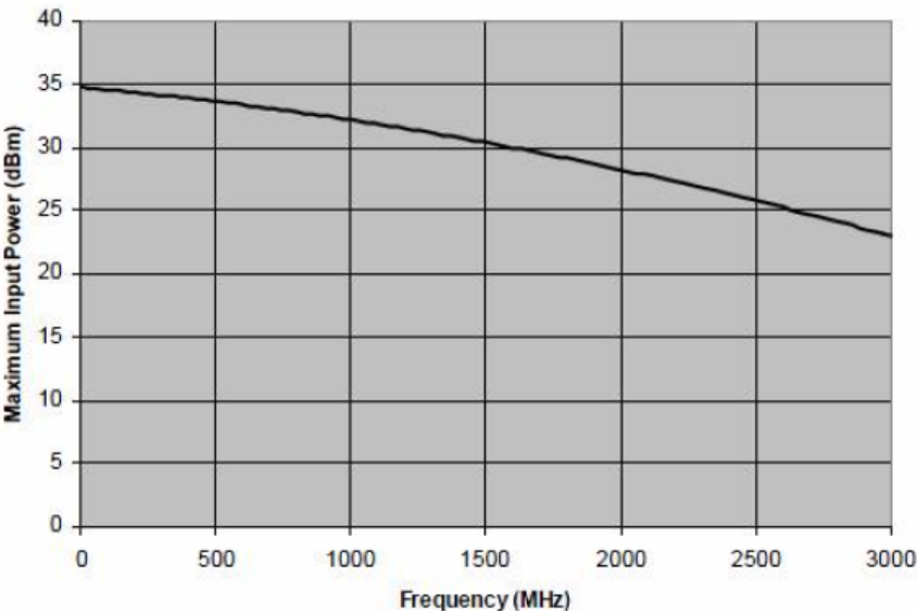
Figure 2. Power derating curve at 25 °C and 3.0V
