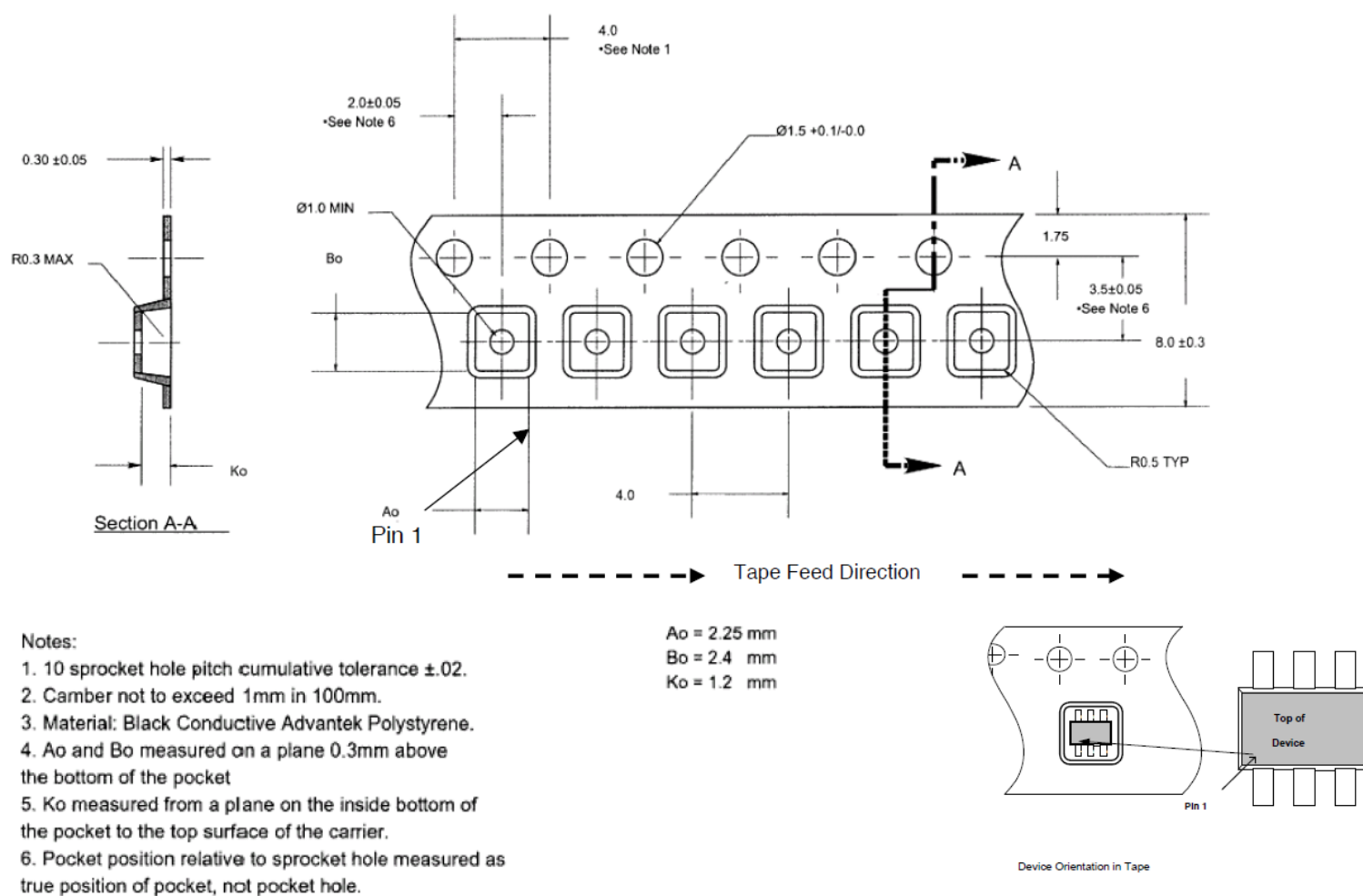
Figure 16. Tape and reel specification for the 6-led SC-70 package
