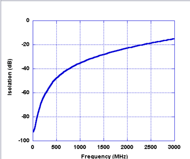
Figure 9. Isolation, output to output
