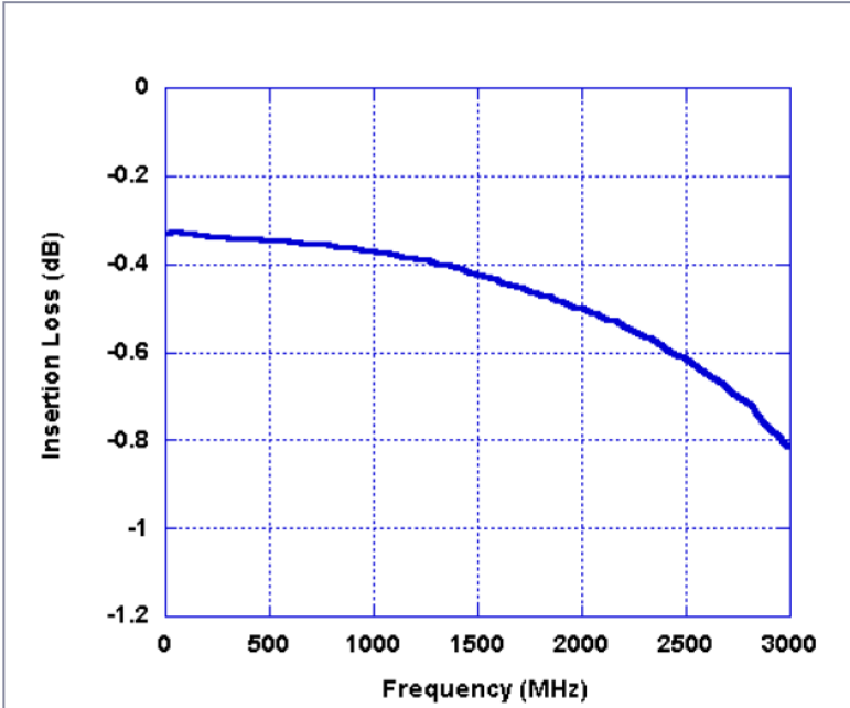
Figure 7. Insertion loss
