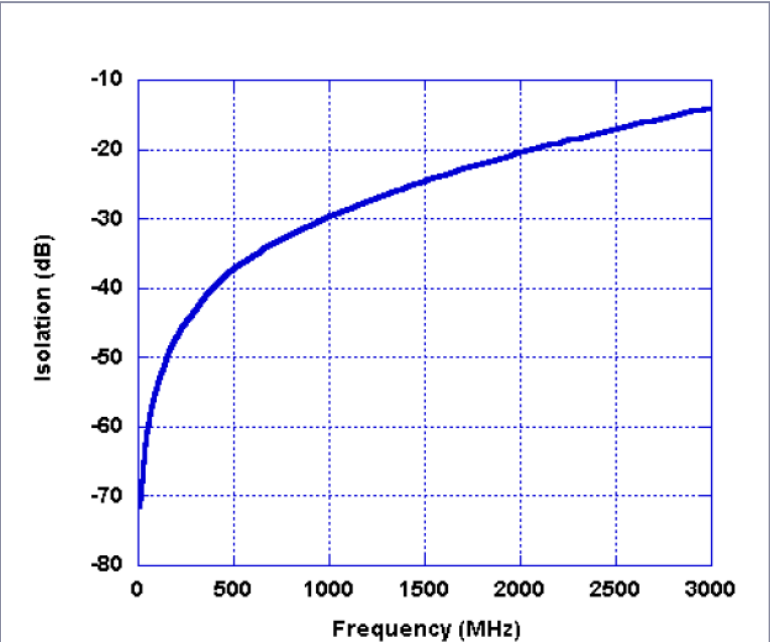
Figure 8. Isolation, input to output
