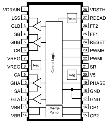
Pinout Diagram
