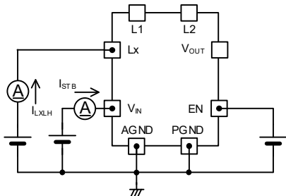
< Circuit No.7 >
