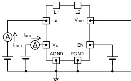
< Circuit No.8 >
