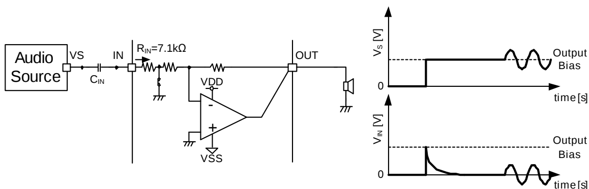
Figure 30. Input voltage transition with input coupling capacitor
