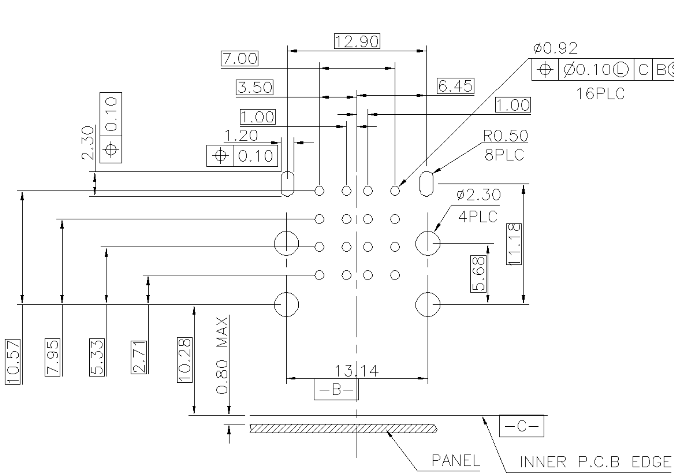
RECOMMENDED P.C.B. LAYOUT (2) (THICKNESS=1.6mm) (GENERAL TOLERANCE: ±0.05)
