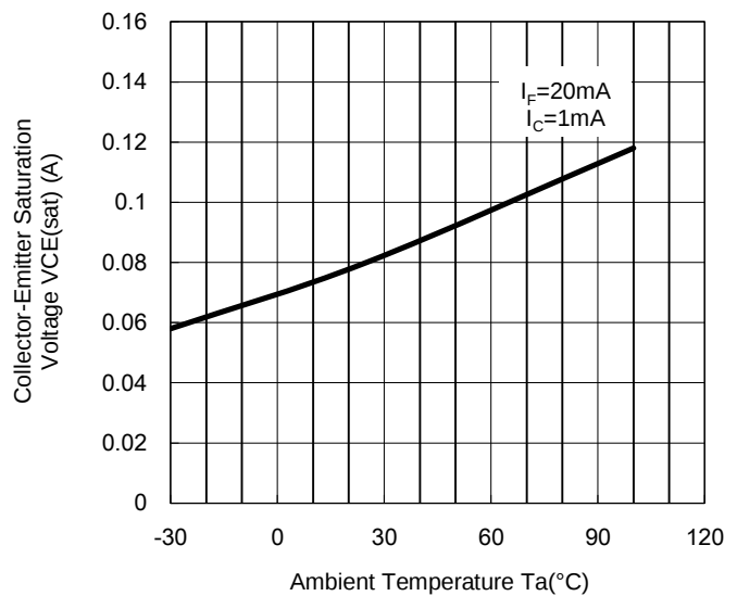
Fig. 8 Collector-emitter Saturation Voltage vs Ambient Temperature
