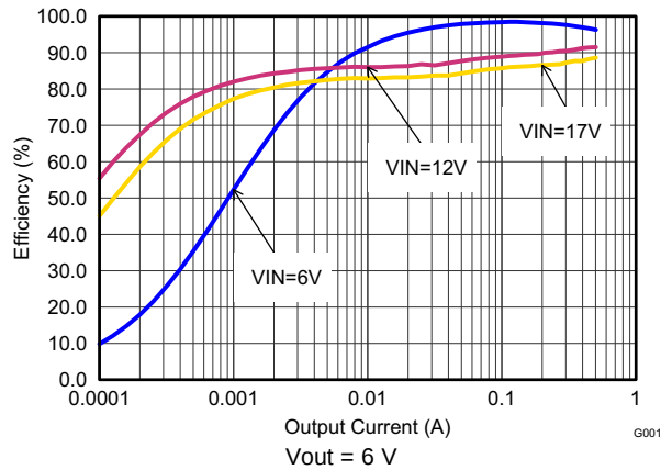
Figure 6. Efficiency versus Output Current
