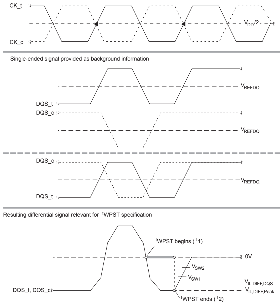
Figure 156: t_{WPST} Method for Calculating Transitions and Endpoints
