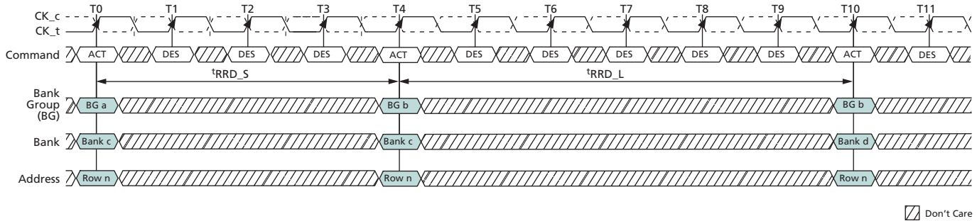
Figure 71: t_{RRD} Timing
