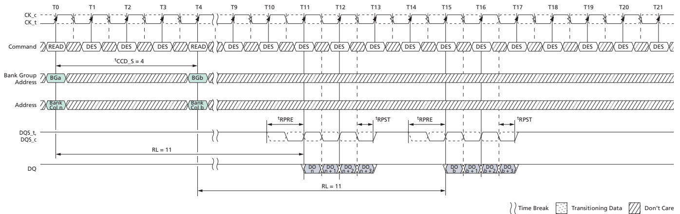
Figure 126: READ (BC4) to READ (BC4) with 1 st CK Preamble in Different Bank Group
