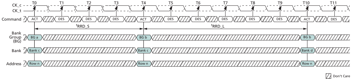
Figure 111: t_{RRD} Timing
