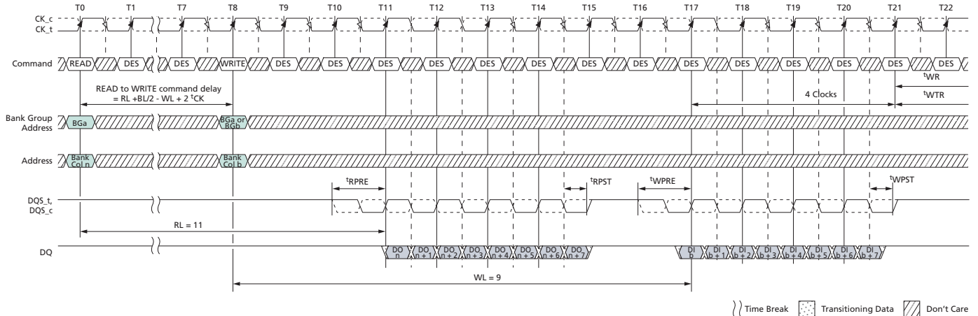
Figure 132: READ (BL8) to WRITE (BL8) with 1 t CK Preamble in Same or Different Bank Group
