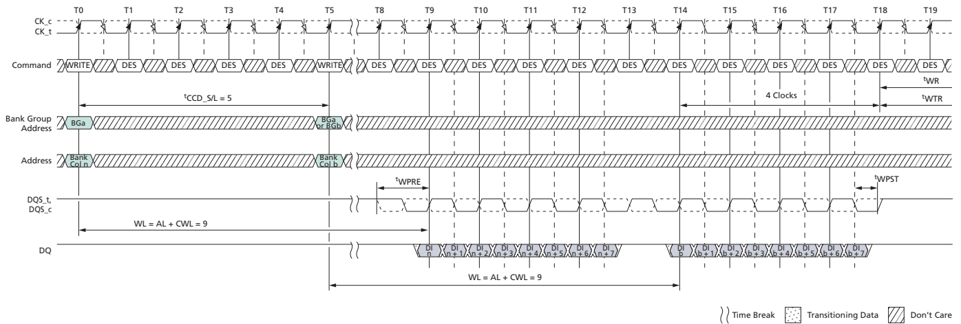
Figure 166: Nonconsecutive WRITE (BL8) with 1 st CK Preamble in Same or Different Bank Group
