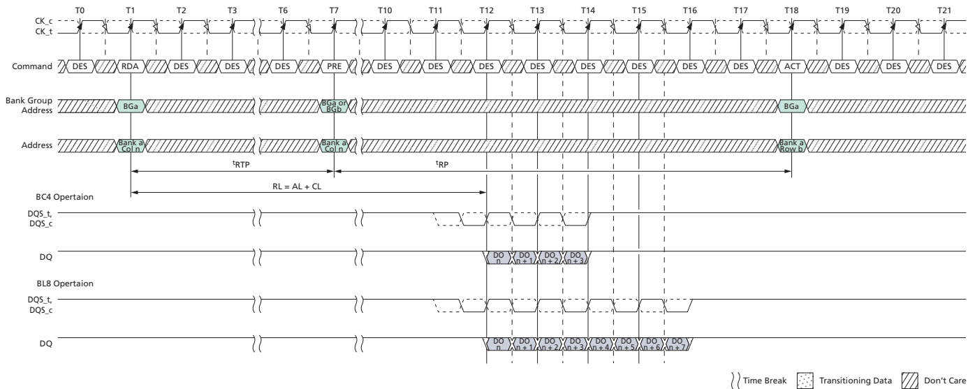
Figure 145: READ with Auto Precharge and 1^{tCK} Preamble
