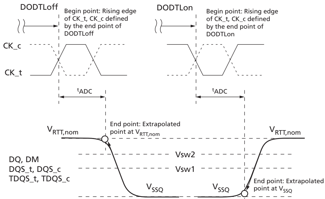
Figure 231: t_{ADC} Definition with Direct ODT Control
