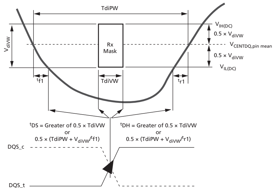
Figure 203: Rx Mask Relative to t DS/ t DH
