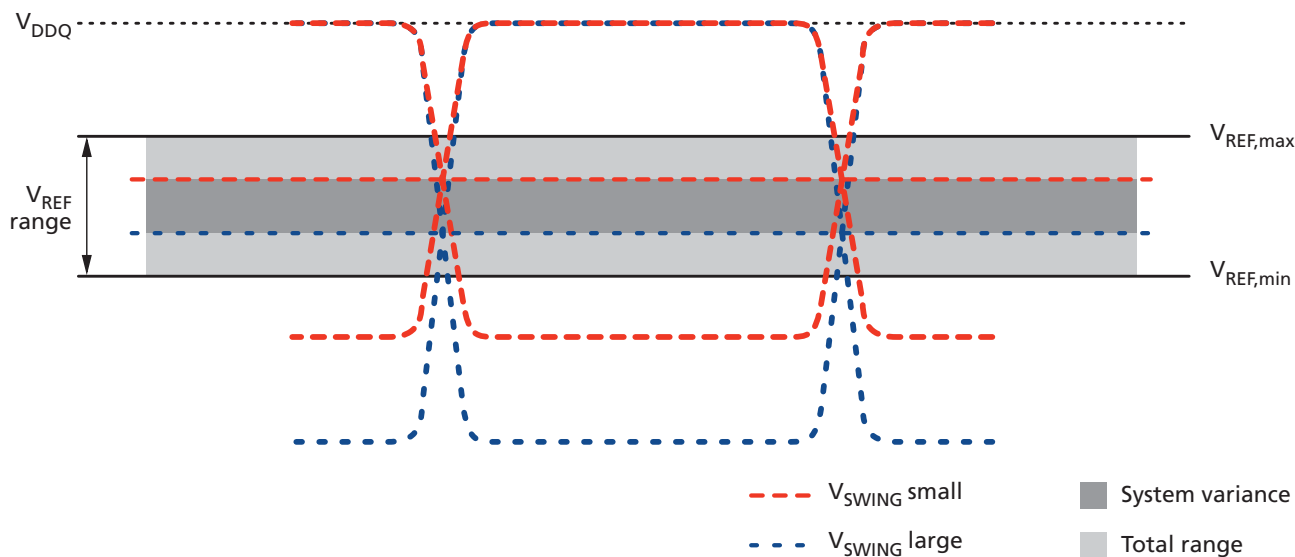
Figure 55: V_{\text{REFDQ}} Voltage Range
