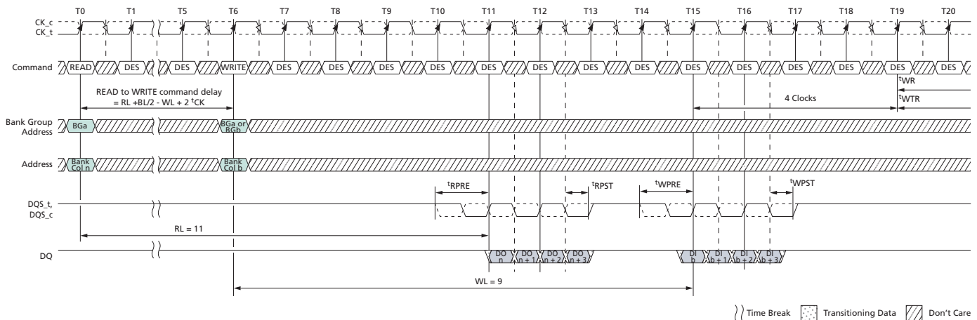
Figure 134: READ (BC4) OTF to WRITE (BC4) OTF with 1^t\text{CK} Preamble in Same or Different Bank Group
