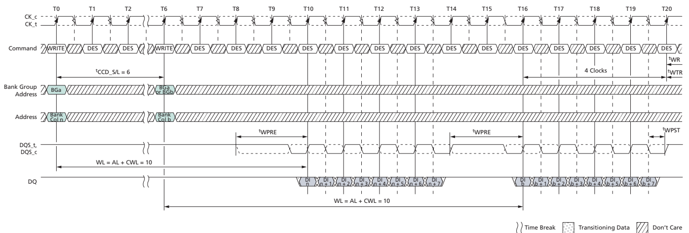
Figure 167: Nonconsecutive WRITE (BL8) with 2 nd CK Preamble in Same or Different Bank Group
