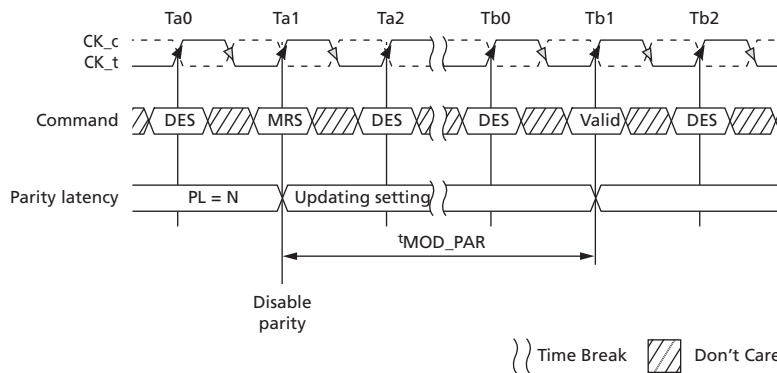
Figure 50: Parity Exit Timing Example – t_{MOD\_PAR}
