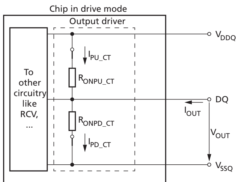
Figure 226: Output Driver During Connectivity Test Mode
