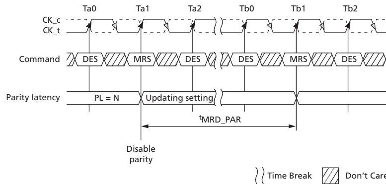
Figure 49: Parity Exit Timing Example – t_{MRD\_PAR}
