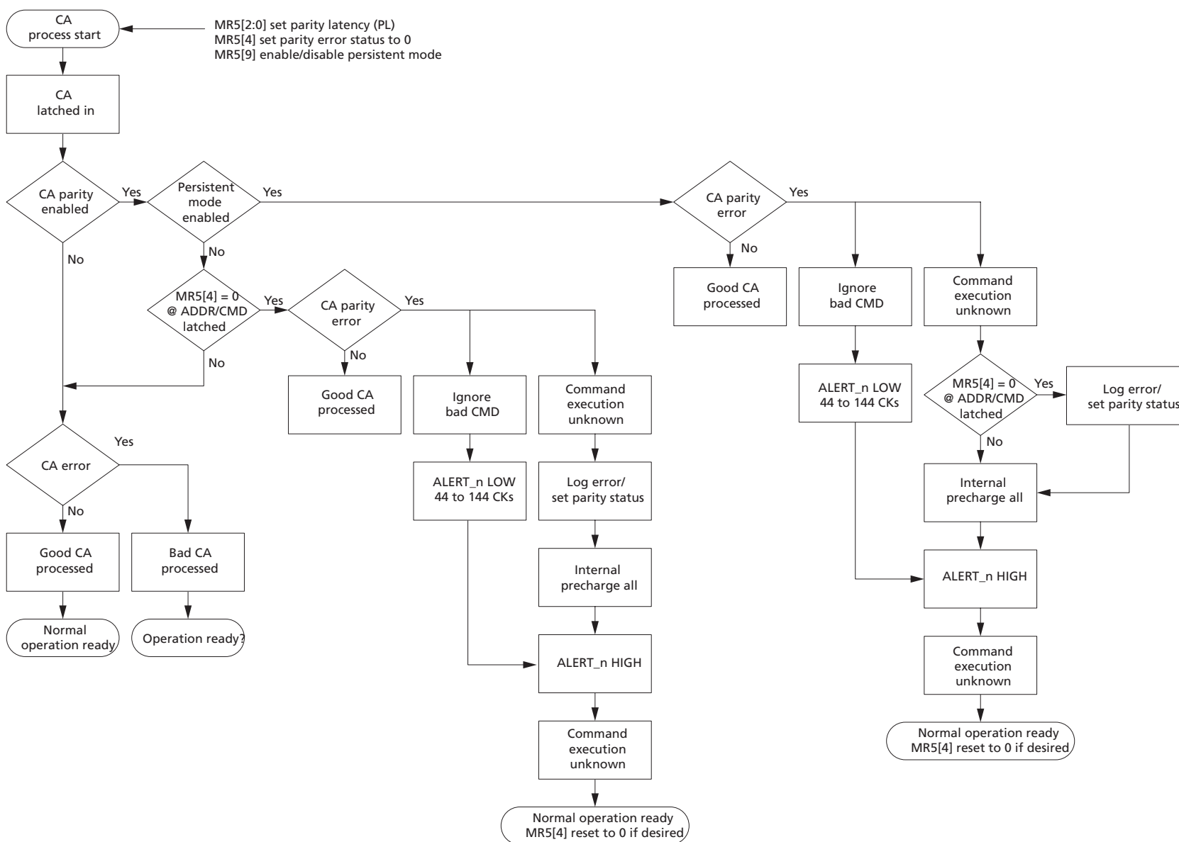
Figure 51: CA Parity Flow Diagram
