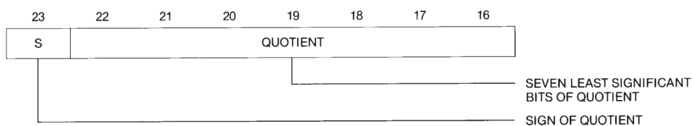
Figure 8-5. Quotient Byte
