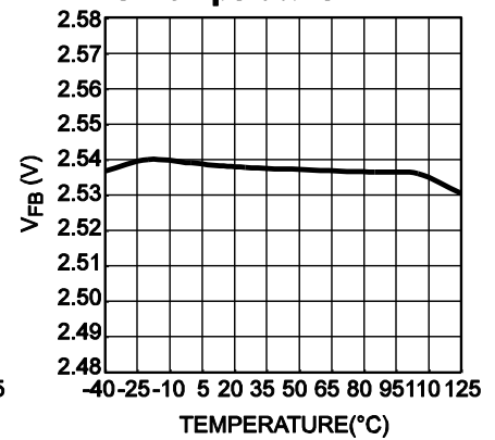
Feedback Threshold vs. Temperature
