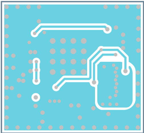
Figure 26: Mid layer 2
