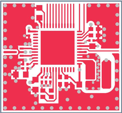
Figure 24: Top layer
