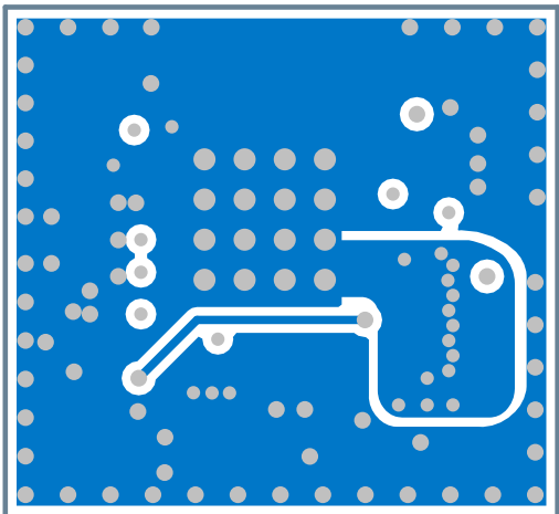
Figure 27: Bottom layer
