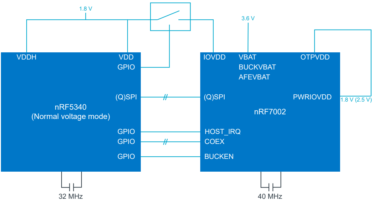
Figure 20: Supply system - normal voltage mode
