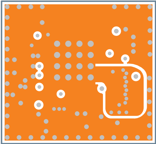
Figure 25: Mid layer 1
