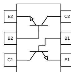
Figure 2. FFB3904 Internal Connection
