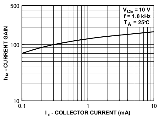
Figure 21. Current Gain
