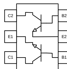
Figure 4. FMB3904 Internal Connection
