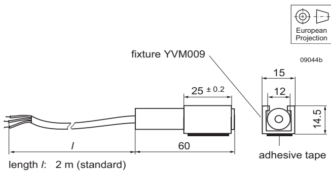
Fig. 57 Mechanical dimensions (in mm)
