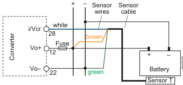
Fig. 55 Wiring diagram sensor
