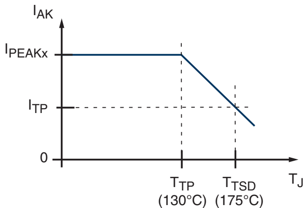
Figure 14. Peak Regulating Current vs. T_J
