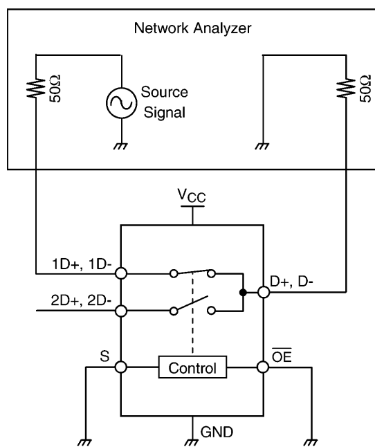
Fig. 11.8 -3dB Bandwidth
