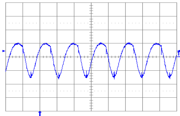
Fig. 3.3V.6: Output voltage ripple (20 mV/div.) at full rated load current into a resistive load with external capacitance 10 \mu F ceramic + 1 \mu F ceramic and V_{in} = 5 V for V_{out} = 3.3 V. Time scale: 2 \mu s/div.
