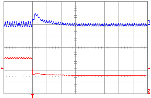
Fig. 1.0V.8: Output voltage response for V_{out} = 1.0\text{ V} to negative load current step change from 5 A to 2.5 A with slew rate of -5 A/ \mu\text{s} at V_{in} = 5\text{ V} . Top trace: output voltage (100 mV/div.); Bottom trace: load current (2 A/div.). C_o = 47\text{ }\mu\text{F} ceramic + 1 \mu\text{F} ceramic. Time scale: 20 \mu\text{s} /div.
