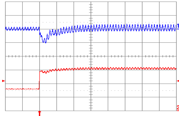
Fig. 1.0V.7: Output voltage response for V_{out} = 1.0\text{ V} to positive load current step change from 2.5 A to 5 A with slew rate of 5 A/ \mu\text{s} at V_{in} = 5\text{ V} . Top trace: output voltage (100 mV/div.); Bottom trace: load current (2 A/div.). C_o = 47\text{ }\mu\text{F} ceramic + 1 \mu\text{F} ceramic. Time scale: 20 \mu\text{s} /div.
