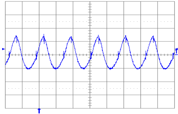
Fig. 1.2V.6: Output voltage ripple (20 mV/div.) at full rated load current into a resistive load with external capacitance 10 \mu F ceramic + 1 \mu F ceramic and V_{in} = 5 V for V_{out} = 1.2 V. Time scale: 2 \mu s/div.
