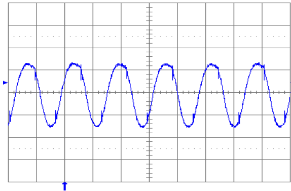
Fig. 2.5V.5: Output voltage ripple ( 20\text{ mV/div.} ) at full rated load current into a resistive load with external capacitance 10\text{ }\mu\text{F} ceramic + 1\text{ }\mu\text{F} ceramic and V_{in} = 5\text{ V} for V_{out} = 2.5\text{ V} . Time scale: 2\text{ }\mu\text{s/div.}
