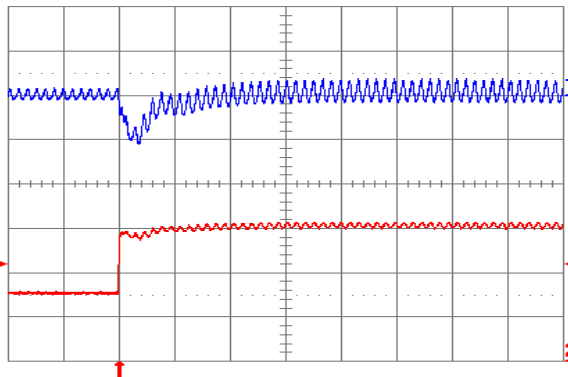
Fig. 1.2V.6: Output voltage response for V_{out} = 1.2 V to positive load current step change from 2.5 A to 5 A with slew rate of 5 A/ \mu s at V_{in} = 5 V. Top trace: output voltage (100 mV/div.); Bottom trace: load current (2 A/div.). C_o = 47 \mu F ceramic + 1 \mu F ceramic. Time scale: 20 \mu s/div.
