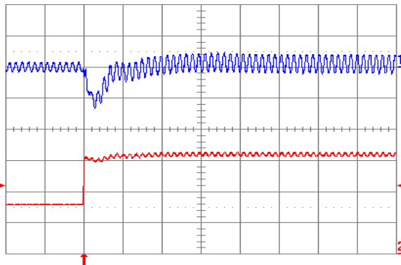
Fig. 2.0V.7: Output voltage response for V_{out} = 2.0 V to positive load current step change from 2.5 A to 5 A with slew rate of 5 A/ \mu\text{s} at V_{in} = 5 V. Top trace: output voltage (100 mV/div.); Bottom trace: load current (2 A/div.). C_o = 47 \mu\text{F} ceramic + 1 \mu\text{F} ceramic. Time scale: 20 \mu\text{s} /div.
