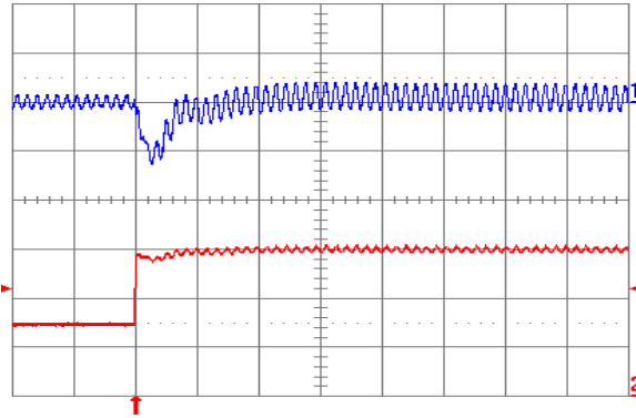
Fig. 1.8V.7: Output voltage response for V_{out} = 1.8V to positive load current step change from 2.5 A to 5 A with slew rate of 5 A/μs at V_{in} = 5V . Top trace: output voltage (100 mV/div.); Bottom trace: load current (2 A/div.). C_o = 47 \mu F ceramic + 1 μF ceramic. Time scale: 20 μs/div.
