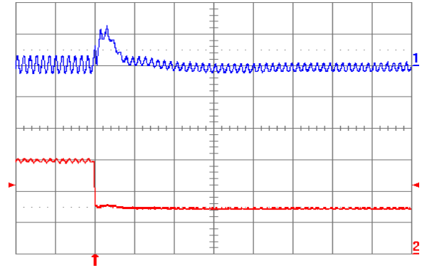
Fig. 1.8V.8: Output voltage response for V_{out} = 1.8V to negative load current step change from 5 A to 2.5 A with slew rate of -5 A/μs at V_{in} = 5V . Top trace: output voltage (100 mV/div.); Bottom trace: load current (2 A/div.). C_o = 47 \mu F ceramic + 1 μF ceramic. Time scale: 20 μs/div.
