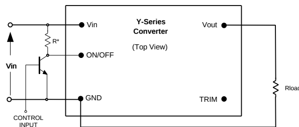
Fig. A: Circuit configuration for ON/OFF function.
