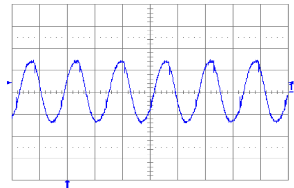
Fig. 1.8V.6: Output voltage ripple (20 mV/div.) at full rated load current into a resistive load with external capacitance 10\text{ }\mu\text{F} ceramic + 1\text{ }\mu\text{F} ceramic and V_{in} = 5\text{ V} for V_{out} = 1.8\text{ V} . Time scale: 2 μs/div.
