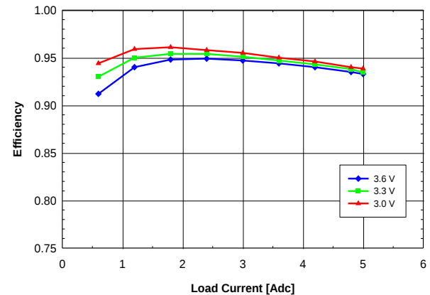
Fig. 2.5V.4: Efficiency vs. load current and input voltage for V_{out} = 2.5\text{ V} converter mounted horizontally with air flowing from pin 5 to pin 1 at a rate of 200 LFM (1 m/s) and T_a = 25\text{ }^{\circ}\text{C} .
