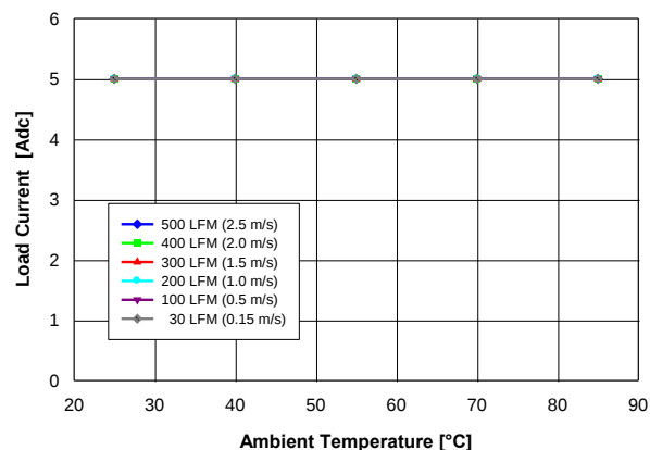
Fig. 1.2V.2: Available load current vs. ambient temperature and airflow rates for V_{out} = 1.2 V converter mounted horizontally with V_{in} = 5 V, air flowing from pin 5 to pin 1 and maximum MOSFET temperature \leq 120 ^{\circ} C.
