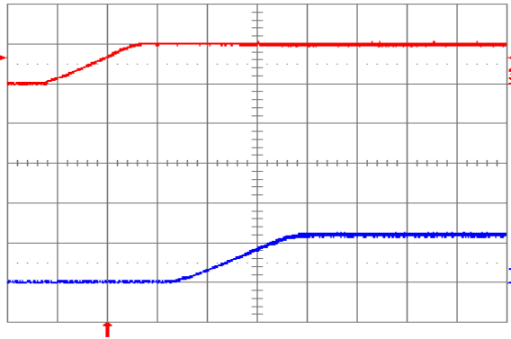
Fig. 1.2V.5: Turn-on transient for V_{out} = 1.2 V with application of V_{in} at full rated load current (resistive) and 47 \mu F external capacitance at V_{in} = 5 V. Top trace: V_{in} (5 V/div.); Bottom trace: output voltage (1 V/div.); Time scale: 2 ms/div.
