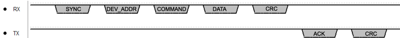
Figure 3. Write command with ACK feedback
