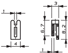
Keying Plug
