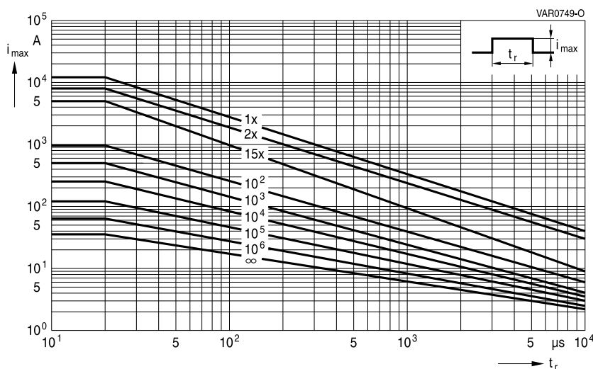
SIOV-SNF20K350 ... K460E3S5K1
