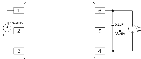
Figure 19 : UVLO Test Circuit
