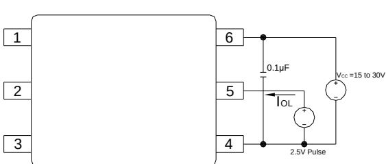
Figure 15 : V_{OL} Test Circuit
