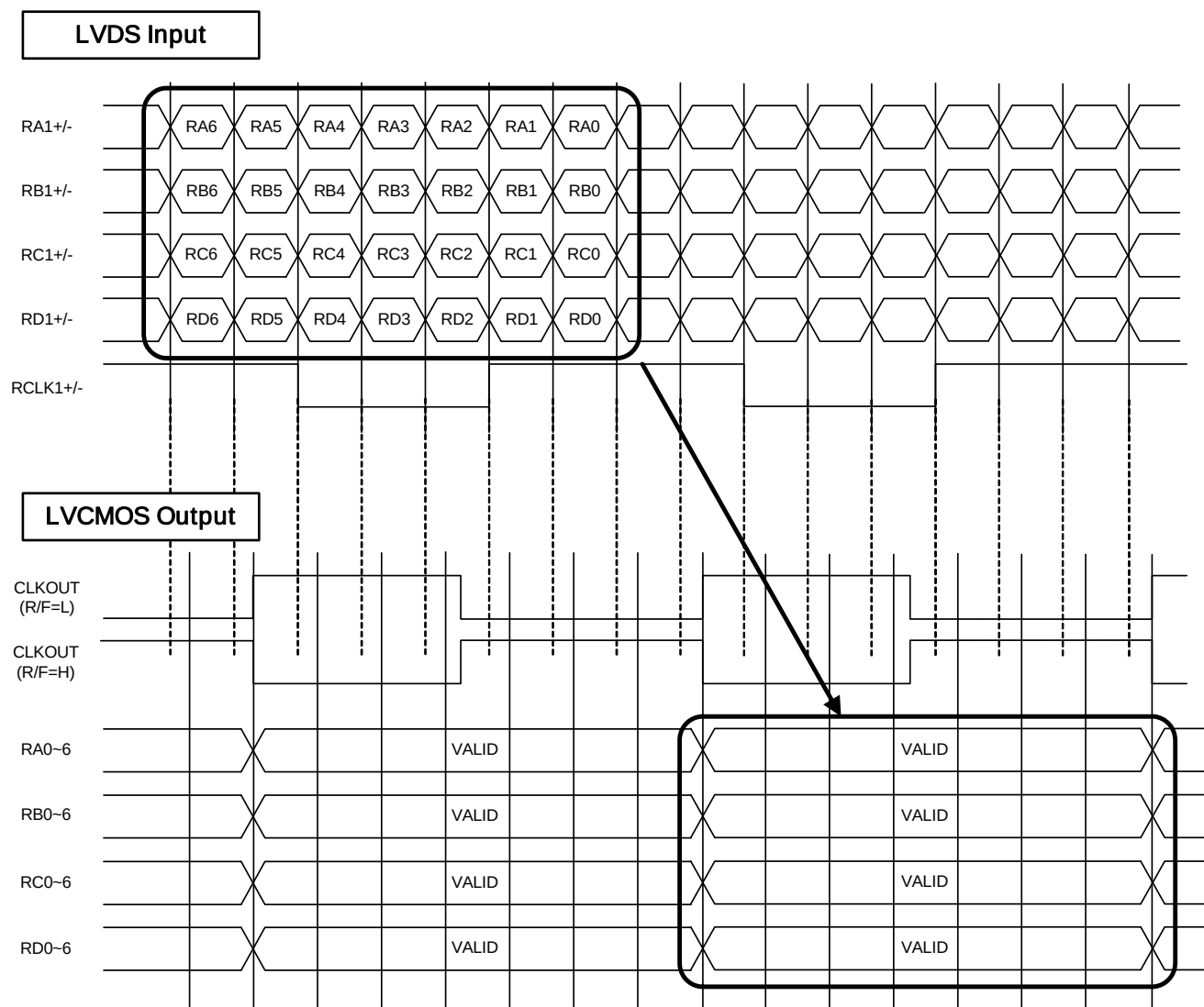
Fig.10 LVDS Data, Clock Input and Output Timing
