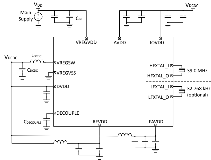
Figure 5.3. EFR32BG26 Typical Application Circuit: DCDC Configuration with PAVDD, RFVDD, AVDD, and IOVDD from DCDC Output
