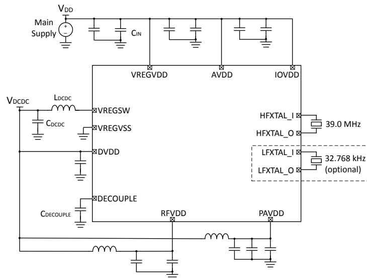
Figure 5.2. EFR32BG26 Typical Application Circuit: DCDC Configuration, PAVDD and RFVDD from DCDC Output, AVDD, and IOVDD from Main Supply
