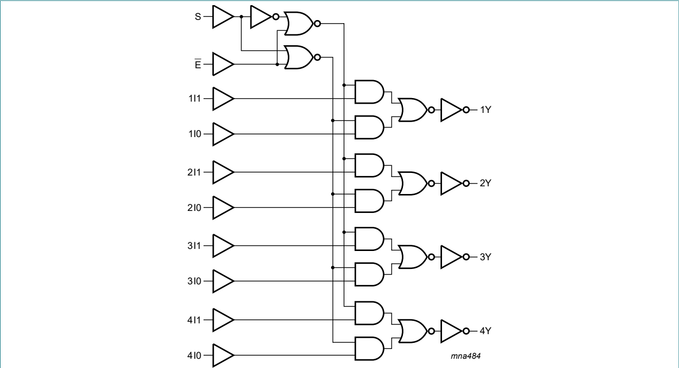
Fig. 4. Logic diagram
