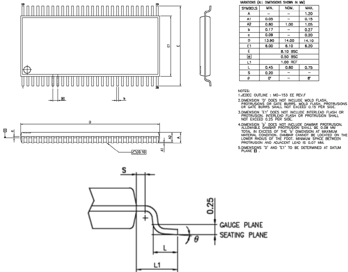
Figure 15. Package Diagram
