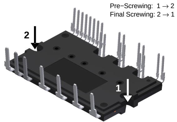
Figure 6. Mounting Screws Torque Order
