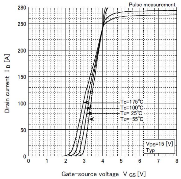
Transfer characteristics
