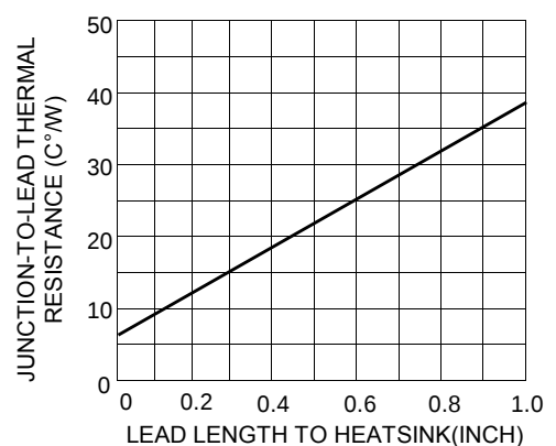
Fig. 2 TYPICAL THERMAL RESISTANCE
