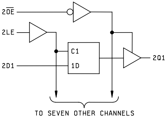
FIGURE 4. Logic diagram.
