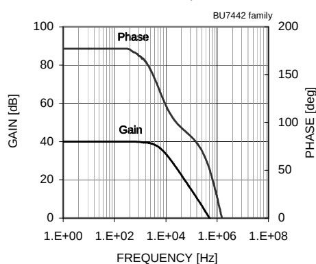
Fig.138 Gain – Frequency
