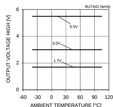
Fig.98 Output Voltage High – Ambient Temperature ( R_L=10[k\Omega] )
