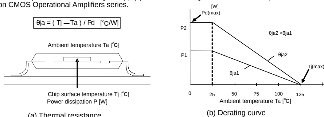
Fig.195 Thermal resistance and derating
