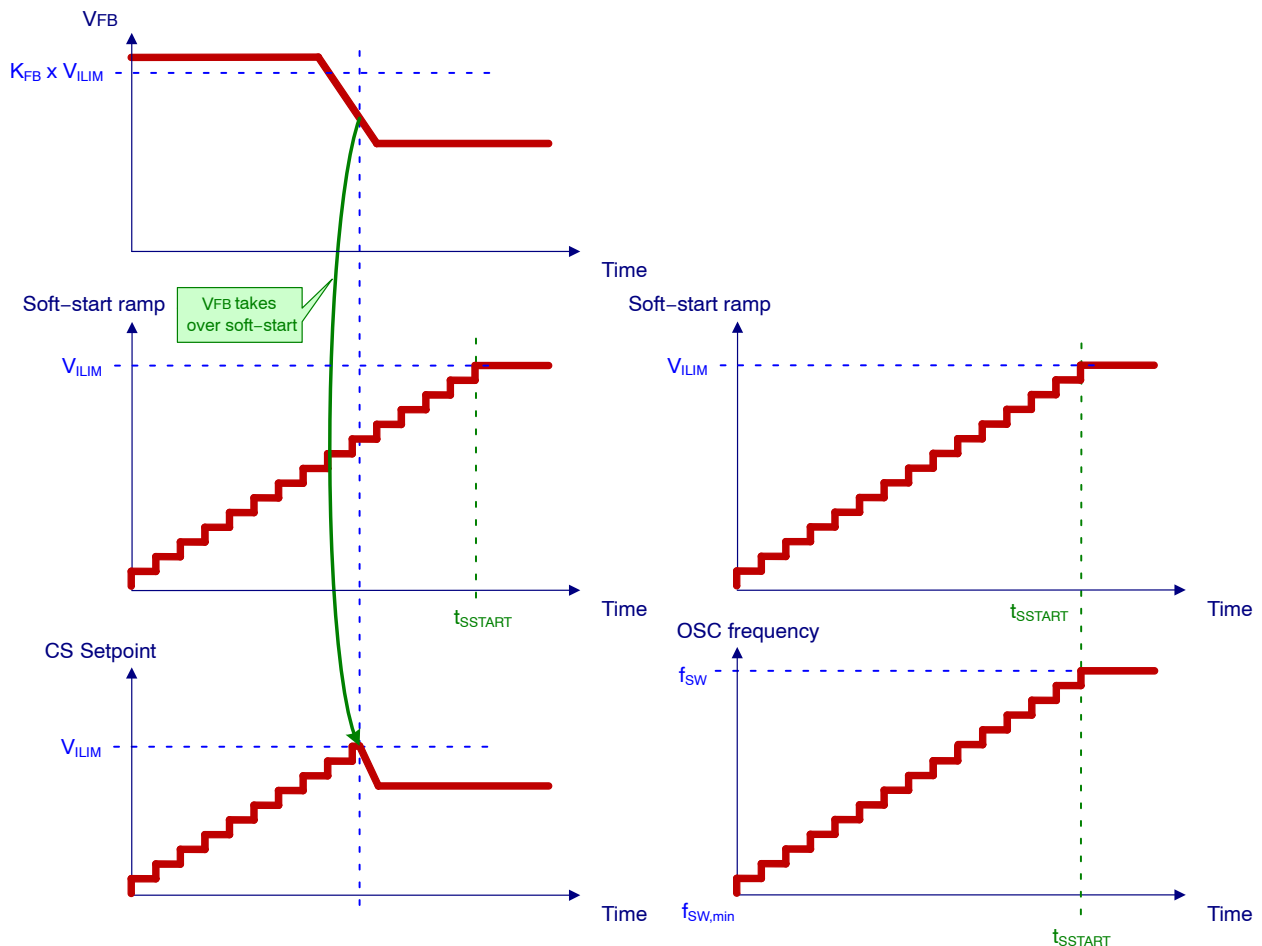
Figure 60. Soft-start Feature
