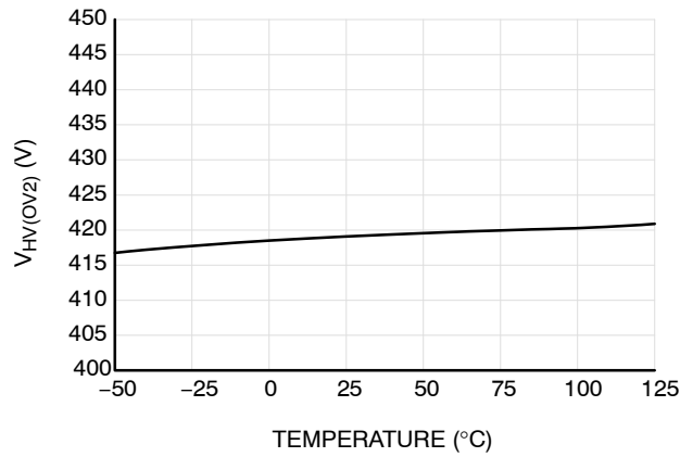
Figure 11. Overvoltage Protection Release Threshold on HV pin V_{HV(OV2)}
