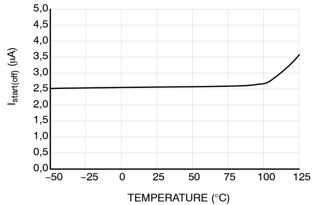
Figure 4. Off-state Leakage Current from HV Pin I_{start(off)}
