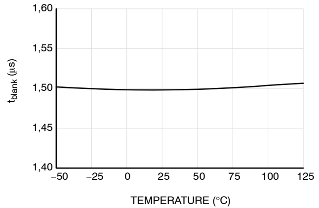
Figure 28. Blanking Time to ZCD OVP Detection after DRV off Event t_{blank}
