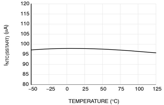
Figure 47. Current I_{NTC(SSSTART)} Sourced Out of the OTP Pin during Soft-start Period
