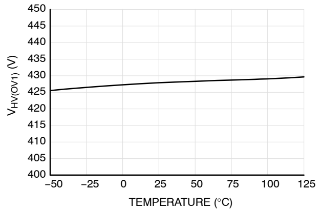
Figure 10. Overvoltage Protection Triggering Threshold on HV Pin V_{HV(OV1)}
