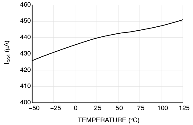
Figure 39. Internal Current Consumption in Fault I CC4
