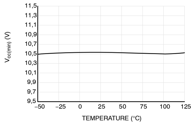
Figure 33. HV Current Source Restart Threshold V CC(min)
