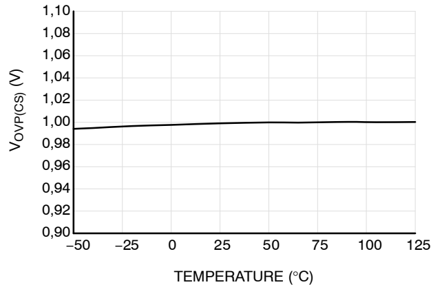
Figure 15. Overvoltage Protection Threshold at CS Pin V OVP(CS)
