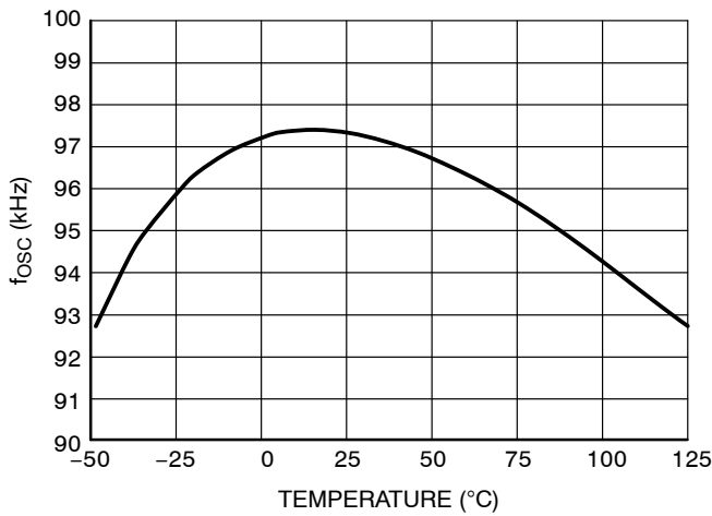
Figure 23. Oscillator f_{osc} for the 65 kHz Version (NCP1240A/B only)
