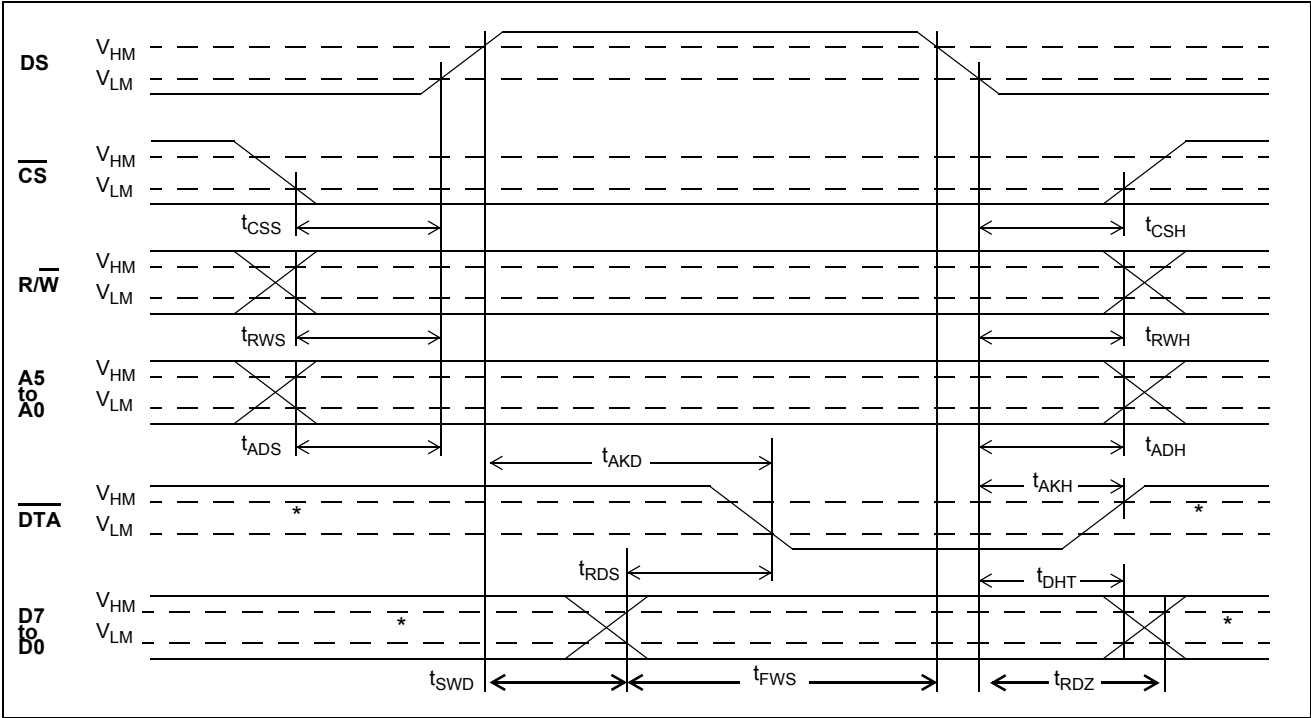
Figure 14 - Processor Bus
