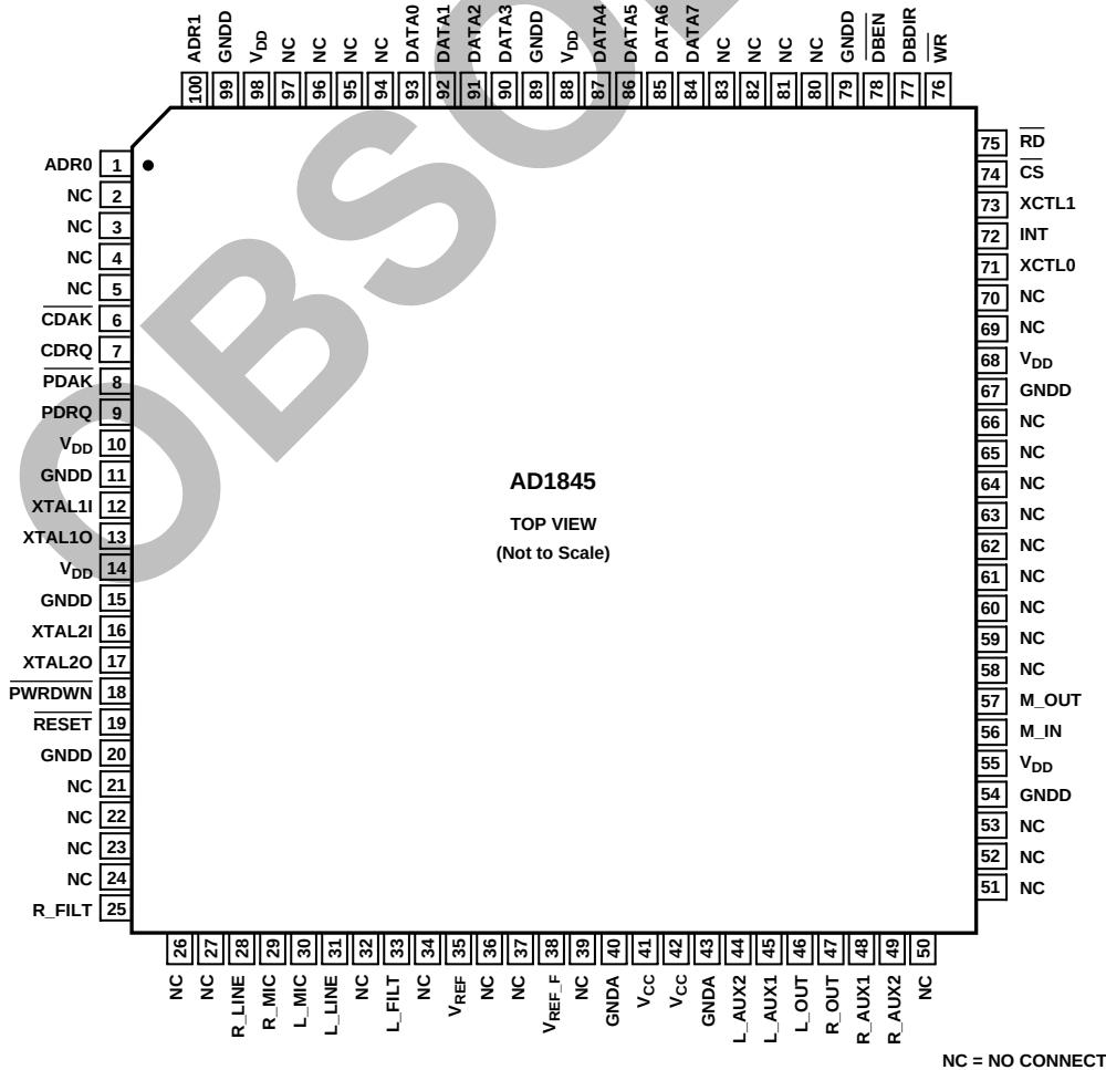
100-Lead TQFP
