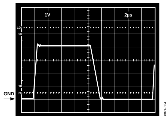
Figure 34. V_S = 5 V, 0 V; Unity-Gain Follower Response to 0 V to 4 V Step
