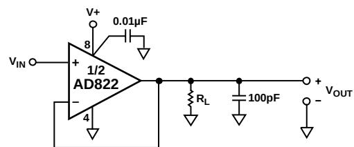
Figure 35. Unity-Gain Follower
