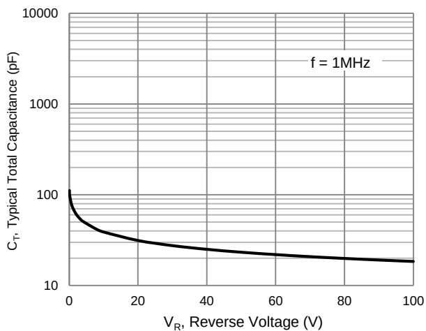
Figure 5. Typical Total Capacitance
