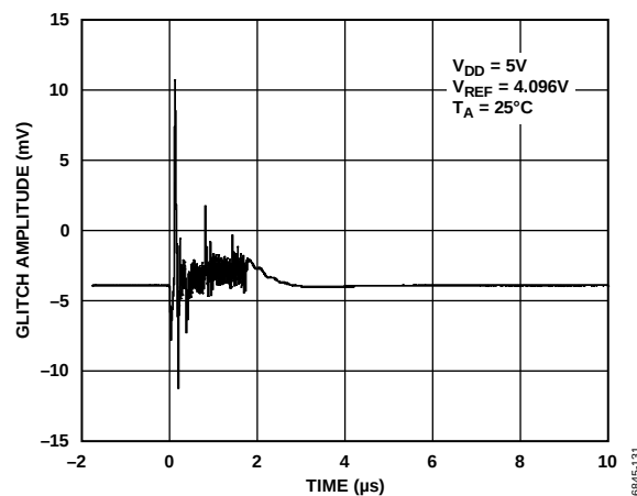
Figure 31. Digital Crosstalk
