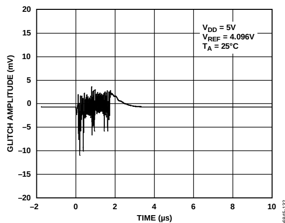
Figure 32. DAC-to-DAC Crosstalk
