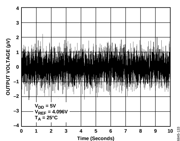
Figure 33. 1/f Noise
