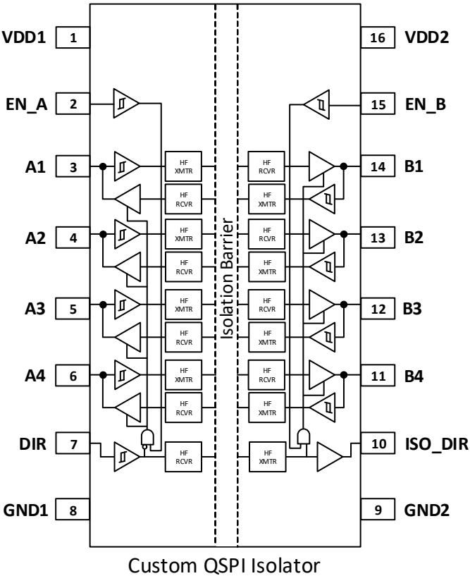
Figure 6. Si86SQ44 Pinout
