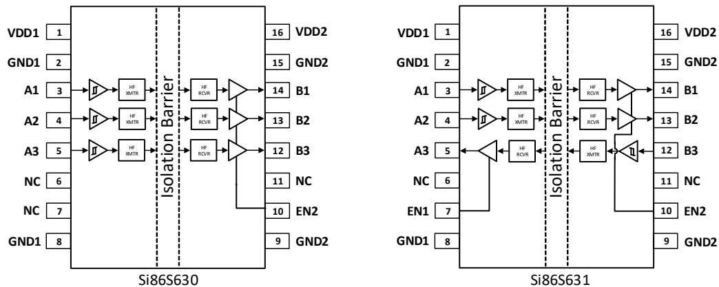
Figure 1. Si86S63x Pinouts
