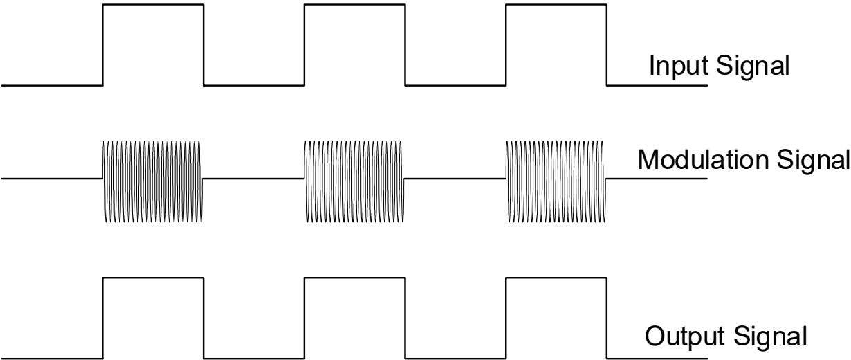
Figure 8. Modulation Scheme
