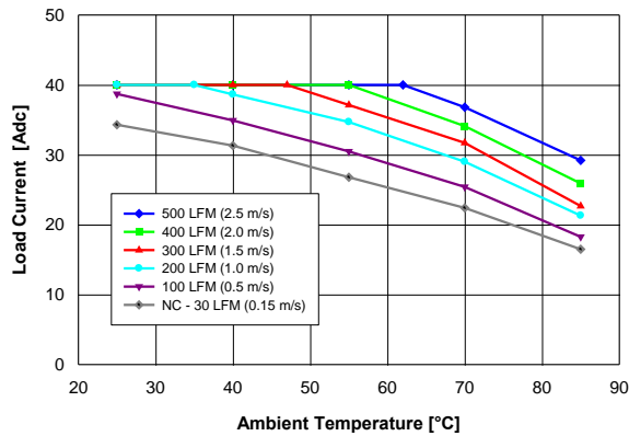
Fig. 1: Available load current vs. ambient air temperature and airflow rates for converter with G height pins mounted vertically with air flowing from pin 1 to pin 3, MOSFET temperature \leq 120^{\circ}\text{C} , V_{in} = 48\text{ V}
