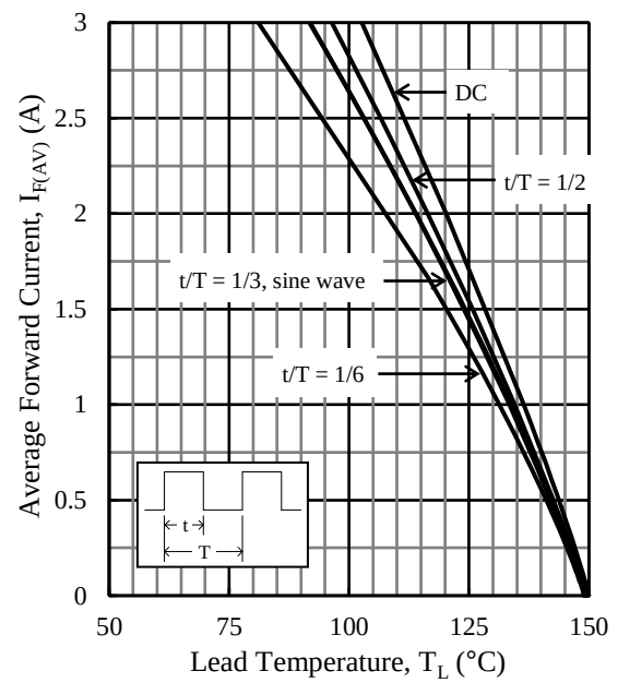
Figure 3. I_{F(AV)} vs. T_L ( T_J = 150 °C, V_R = 200 V)
