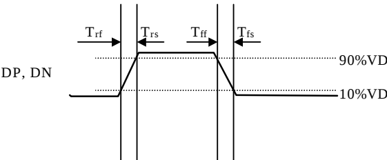
Figure 2. Rise/Fall Time
