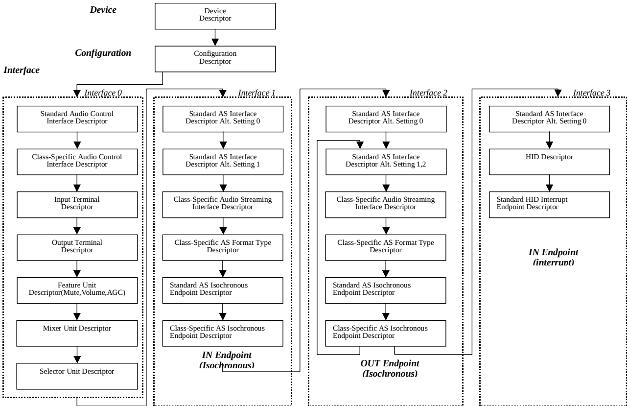
Figure 13 Descriptor Hierarchy
