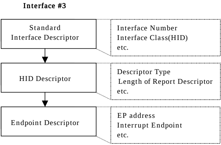
Figure 8 Hierarchy of HID Interface
