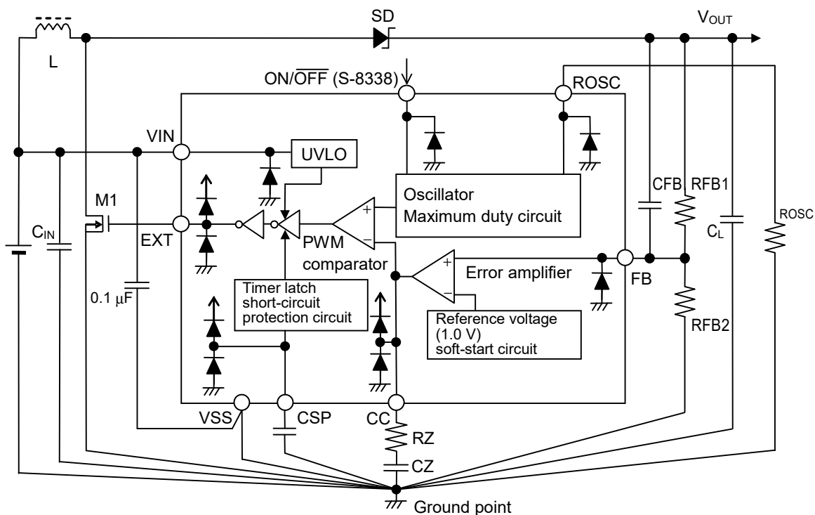
Figure 15 Standard Circuit (S-8338 Series)
