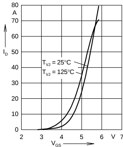
Fig. 4 Typ. transfer characteristics I_D = f(V_{GS}) (MOSFET)
