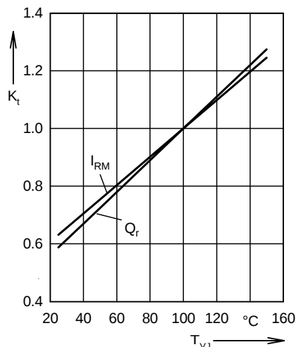
Fig. 13 Dynamic parameters versus junction temperature (Boost Diode)
