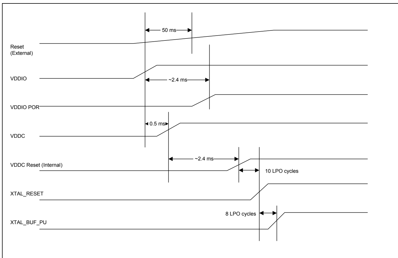
Figure 2. Reset Timing
